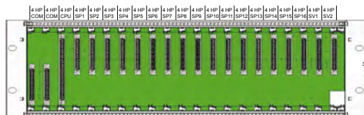
19" Basic unit II
